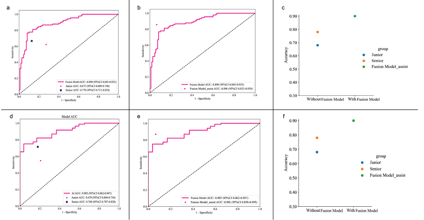
SUPPLEMENTARY FIG. 3. Diagnostic performance and comparison of radiologists with and without the fusion model in external validation cohort 1 and validation cohort 2. AUC, area under the curve; CI, confidence interval.
